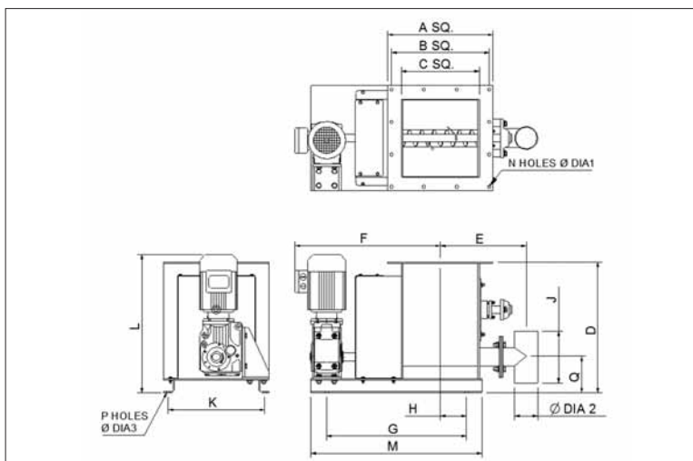
Dosing Screws
